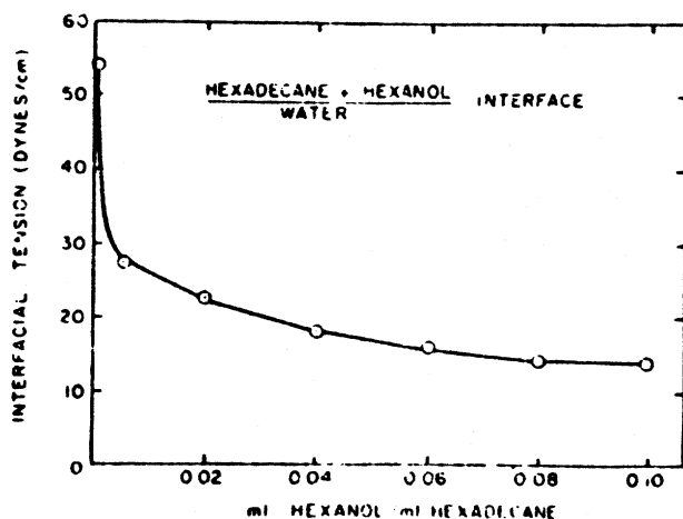
Fig. 1. The effect of hexanol on interfacial tension of hexadecane/water interface.
