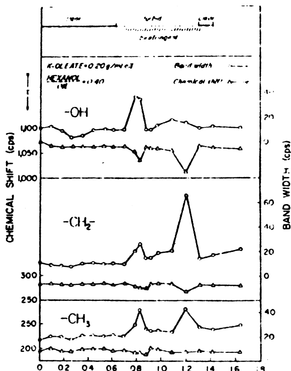
Fig. 4. Variation in the band width at half height and chemical shift of water and hexanol ( -\text{OH} ), methylene ( -\text{CH}_2- ), and methyl ( -\text{CH}_3 ) protons in high resolution NMR (220-megacycle) spectra of the same microemulsions as that in Figure 3, as the water content increases. The upper part of the diagram shows corresponding data on optical clarity and birefringence.
