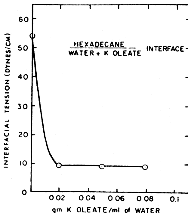
Fig. 2. The effect of potassium oleate on interfacial tension of hexadecane/water interface.
