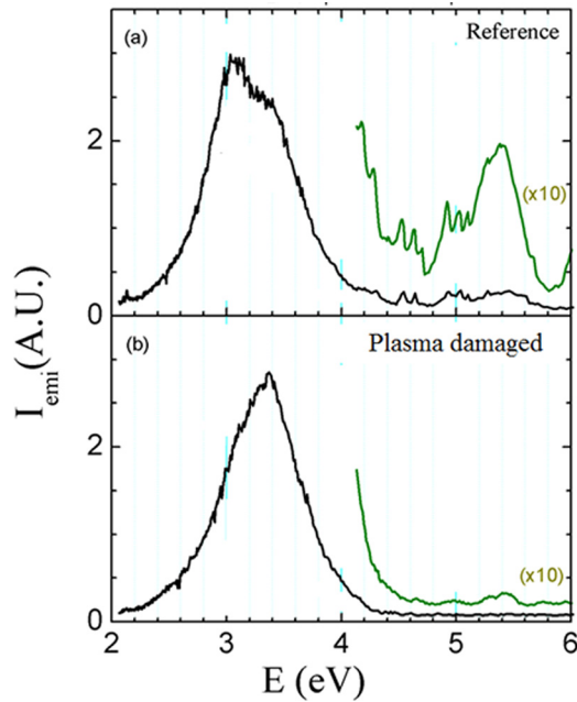
FIG. 5. (Color online) Comparison of 10 K photoluminescence of spectra of (a) a reference \text{Ga}_2\text{O}_3 sample and (b) a plasma damaged \text{Ga}_2\text{O}_3 sample. The higher energy peaks exhibit the spectra measured in the higher sensitivity range and are enlarged for clarity.
