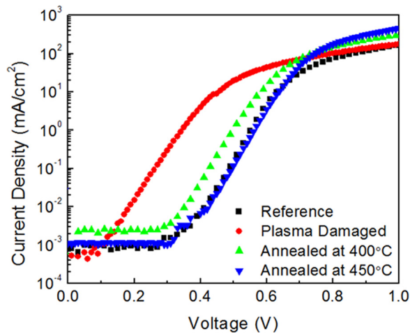
Fig. 2. (Color online) Forward I–V characteristics of Ni/Au \text{Ga}_2\text{O}_3 diodes on surfaces dry etched in \text{BCl}_3/\text{Ar} ICP discharges and annealed at 400 or 450 °C prior to metallization.
