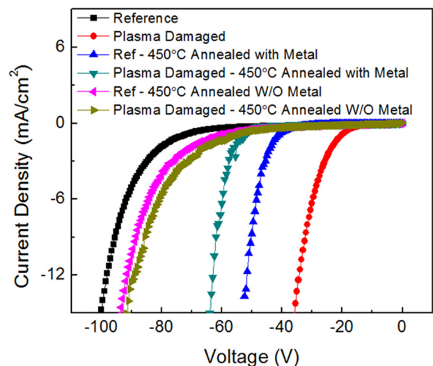
Fig. 4. (Color online) Reverse I–V characteristics of Ni/Au \text{Ga}_2\text{O}_3 diodes on surfaces dry etched in \text{BCl}_3/\text{Ar} ICP discharges and annealed at 450 °C either before or after deposition of Ni/Au.
