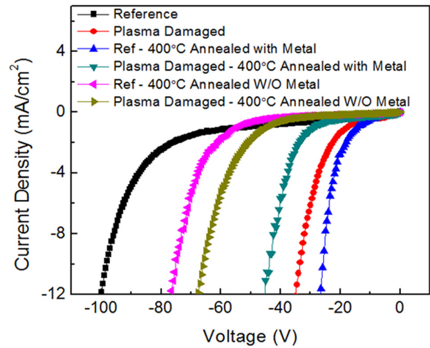
Fig. 3. (Color online) Reverse I–V characteristics of Ni/Au \text{Ga}_2\text{O}_3 diodes on surfaces dry etched in \text{BCl}_3/\text{Ar} ICP discharges and annealed at 400 °C either before or after deposition of Ni/Au.
