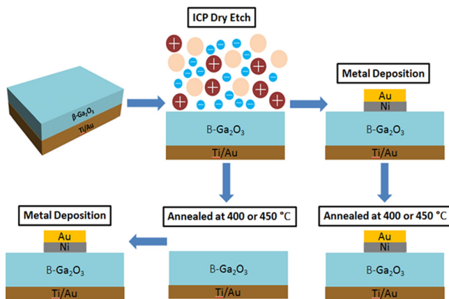
FIG. 1. (Color online) Schematic of experiment-Ni/Au Schottky diodes formed on dry etched \beta -Ga 2 O 3 surfaces either before or after subsequent annealing at 400 or 450 °C.
