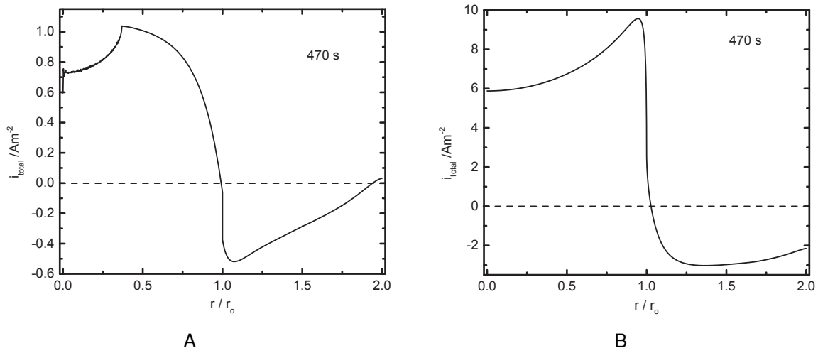
Figure 4-22. The distribution of total current density at t = 470 s for the mechanisms A) proposed by Remita B) proposed by Nordsveen of the CO 2 Deposit model.
