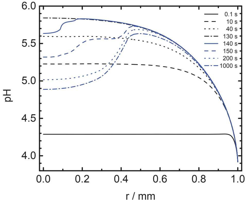
Figure 4-27. The pH distribution as a function of time calculated for the CO 2 Droplet model.
