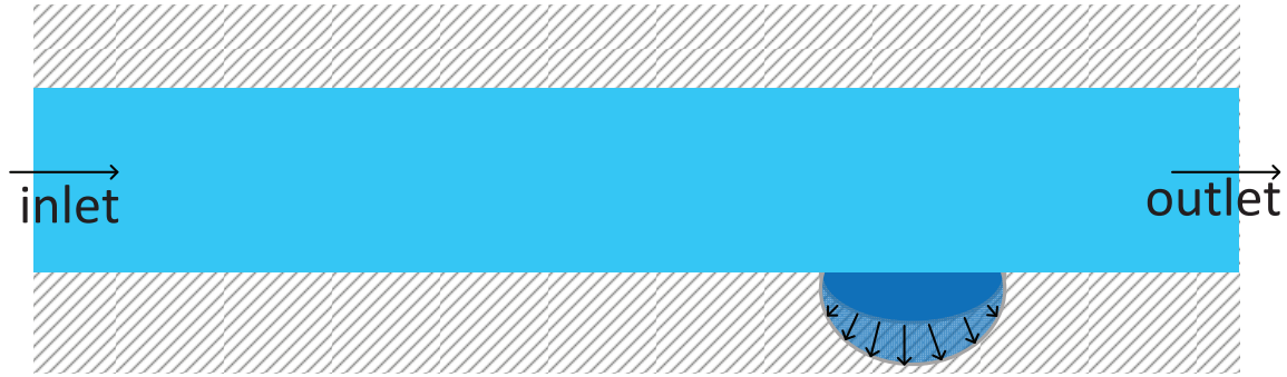
Figure 7-3. Schematic representations of the channel flow model with moving boundary conditions on the predefined defect.
