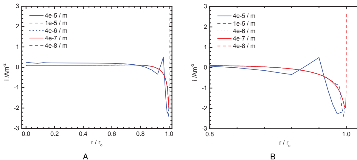
Figure 4-33. Radial distributions of calculated A) total current density and B) the total current density near the periphery region at the electrode surface with time as a parameter for the CO 2 Droplet model.
