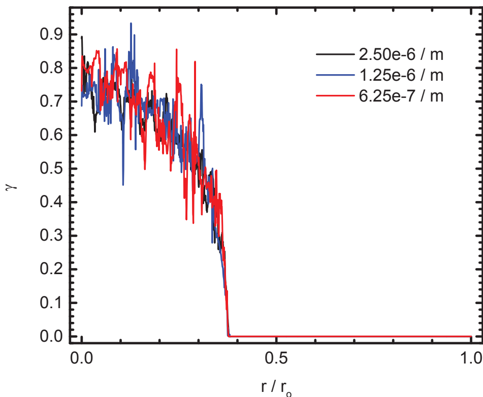
Figure 4-34. Radial distributions of calculated total current density at the electrode surface with maximum mesh element size as a parameter for the CO 2 Droplet model.
