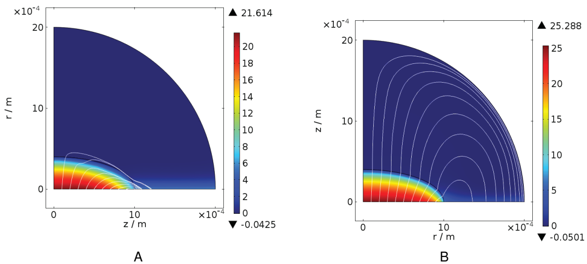
Figure 4-23. The potential distributions at t = 470 s for the mechanisms A) proposed by Remita B) proposed by Nordsveen of the CO 2 Deposit model.
